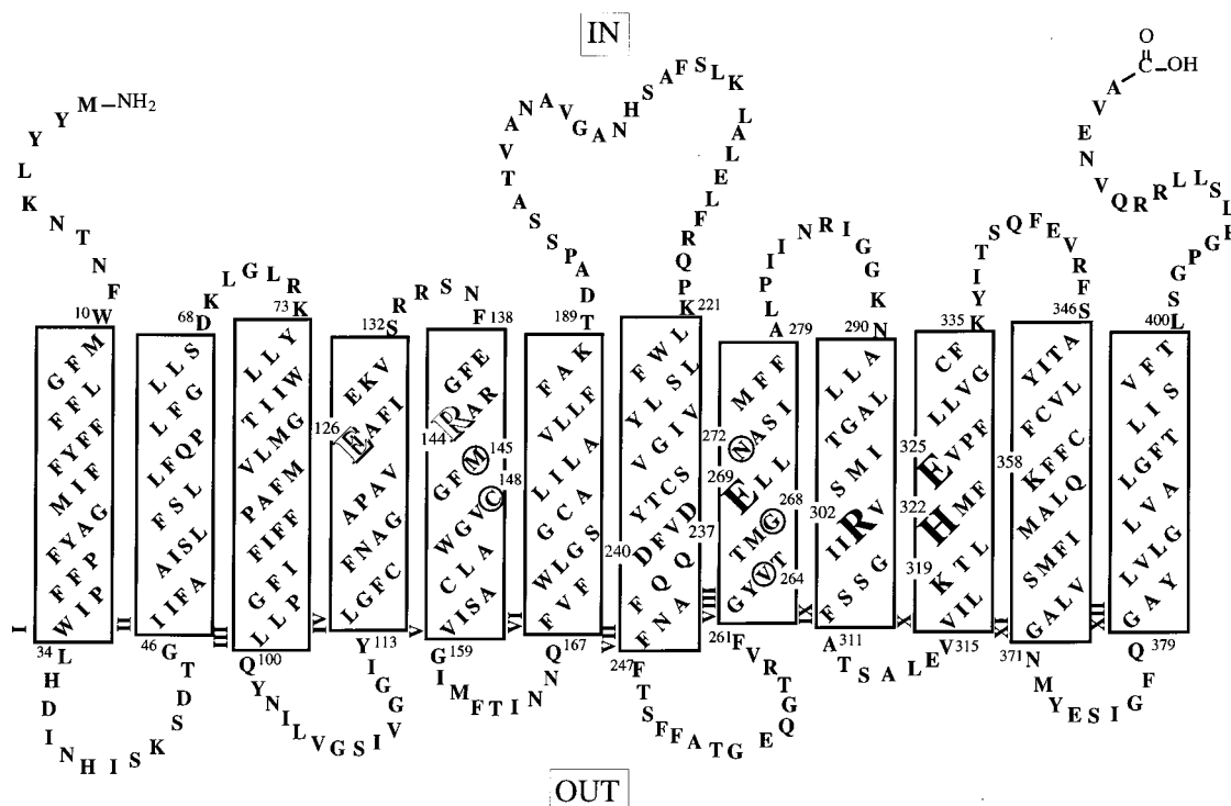
FIGURE 1. Secondary structure model of lacP. The one-letter amino acid code is used, and putative transmembrane helices are shown in boxes. Residues irreplaceable with respect to active transport are enlarged: those involved in substrate translocation are open [Glu126 (helix IV) and Arg144 (helix V)]; those involved in H^+ translocation and coupling are in black [Glu269 (helix VIII), Arg302 (helix IX), His322 (helix X), and Glu325 (helix X)]. Asp237 (helix VII) and Lys358 (helix XI), as well as Asp240 (helix VII) and Lys319 (helix X), which are charge paired, are slightly enlarged and numbered. Nonessential residues thought to be involved in substrate translocation [Met145 and Cys148 (helix V); Val264, Gly268, and Asn272(helix VIII)] are encircled.
