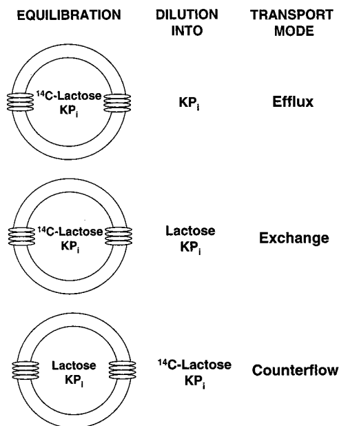
FIGURE 5. Efflux, exchange, and counterflow. To study efflux or equilibrium exchange, concentrated suspensions of right-side-out membrane vesicles are equilibrated passively with radioactive lactose at a final concentration of 10 mM. Aliquots are then diluted 200-fold or more into buffer without (efflux) or with 10 mM cold lactose (equilibrium exchange). For counterflow experiments, concentrated suspensions are equilibrated passively with cold lactose at a final of 10 mM, and aliquots are diluted 200-fold or more into buffer containing radioactive lactose at a final concentration of 0.4 mM. Initially, internal cold lactose exchanges rapidly with external radioactive lactose until all of the internal cold is exchanged, at which point the reaction ceases, the gradients dissipate, and the signal returns to baseline. During each of these operations, care is taken to collapse any \Delta\bar{\mu}_{H^+} that may be generated.
